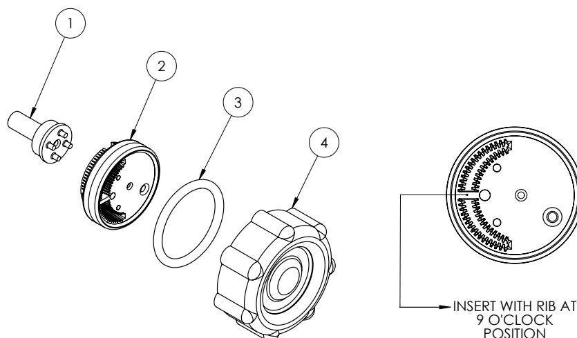
Figure 12: Injector Assembly
